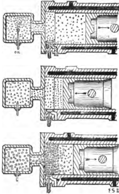
FIG. 223.—Diagram of the Hornsby-Akroyd Ignition System. At the end of the cylinder is a box, or chamber, connected to it by a narrow neck. During the suction stroke, shown in the first figure, air is drawn into the cylinder and oil sprayed into the hot igniting chamber.
